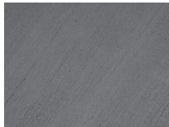
Ironstone
