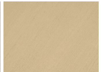
Clay
