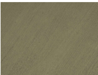
Slate
