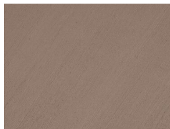
Siltstone
