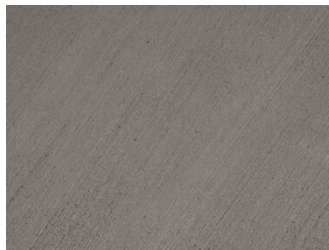
Diorite
